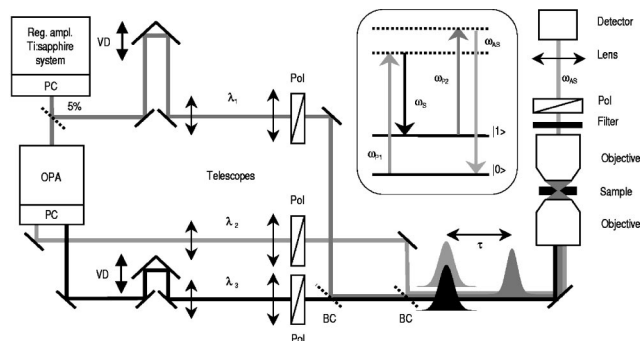
FIG. 1. Schematic of the time-resolved CARS microscope. Inset: Energy diagram of the four-wave mixing process with three incident fields. PC, pulse compression stage; VD, variable delay line; Pol, polarizer; and BC, dichroic beam combiner.
