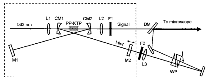
Fig. 1. OPO resonator and external layout used for CARS microscopy. The OPO is singly resonant within the idler beam wavelength range. CM1, CM2, OPO cavity concave ( r=100\text{ mm} ) mirrors with high reflection ( R > 99\% ) in the idler beam wavelength range. CM2 has 70%–80% transmission at the signal beam wavelengths. M1, high-reflecting mirror; M2, 10% output coupler for the idler beam; F1, F2, long-pass filters, > 850\text{ nm} ; L1, L2, L3, lenses with focal lengths of 50, 150, and 1000 mm, respectively; DM, dichroic mirror; WP, wedged plates for delay control.
