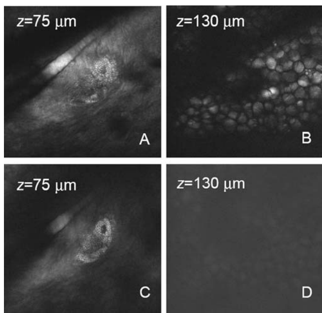
Fig. 4. Forward CARS images of mouse ear tissue at the aliphatic CH 2 stretching frequency, 2850 \text{cm}^{-1} , at two different depths of z=75 \mu\text{m} and z=130 \mu\text{m} , taken with two different sources. A, B, the OPO. C, D, the two picosecond-Ti:sapphire-lasers-based system.
