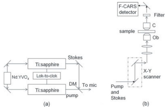
Fig. 1. Schematic of the coherent anti-Stokes Raman scattering (CARS) light source and microscope setup. Nd:YVO4: 1064 & 532 nm laser; DM: dichroic mirror; Ob: 1.2 NA water 60 \times objective lens; C: 0.55 NA air condenser (a) Light source employing two synchronized Ti:sapphire lasers (b) Laser scanning microscope modified for detecting forward CARS (F-CARS) signal.
