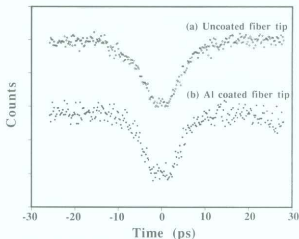
Fig. 3. (a) Experimental data on an uncoated fiber tip (1 m long). (b) Experimental data on an aluminum coated fiber tip. The FWHM of both traces are 10 ps, which is identical to that of the input laser pulses measured with a conventional autocorrelation technique.
